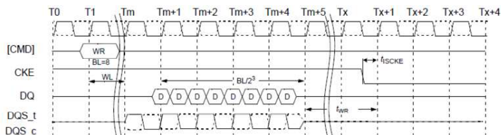
WRITE to Power-Down Entry
