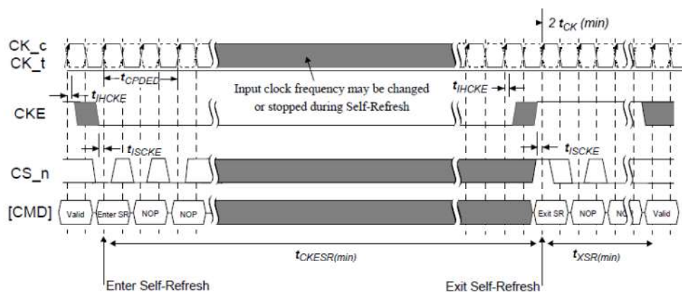
Self-Refresh Operation
