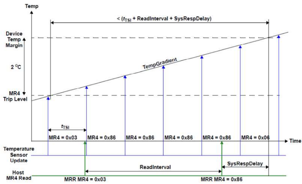
Temp Sensor Timing
